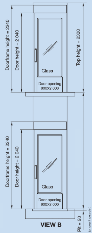
standard layout (section view)*
