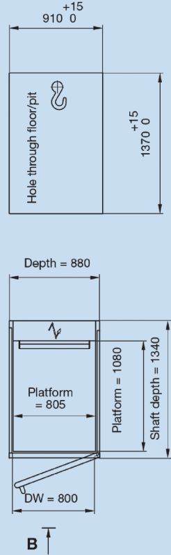
standard layout (plan view)*
